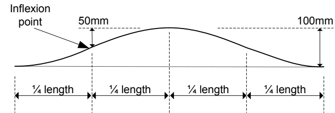
Detail of sinusoidal hump profile
